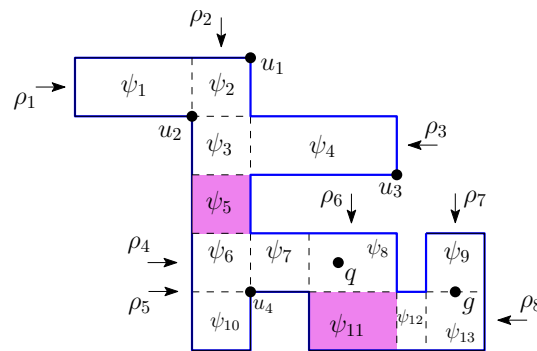
■ Figure 1 A tree polygon with pixels \{\psi_1, \dots, \psi_{13}\} and maximal axis-aligned rectangles \{\rho_1, \dots, \rho_8\} ; rectangle \rho_5 is degenerate. Pixel-guard \psi_5 guards u_3 via its top-right corner.
